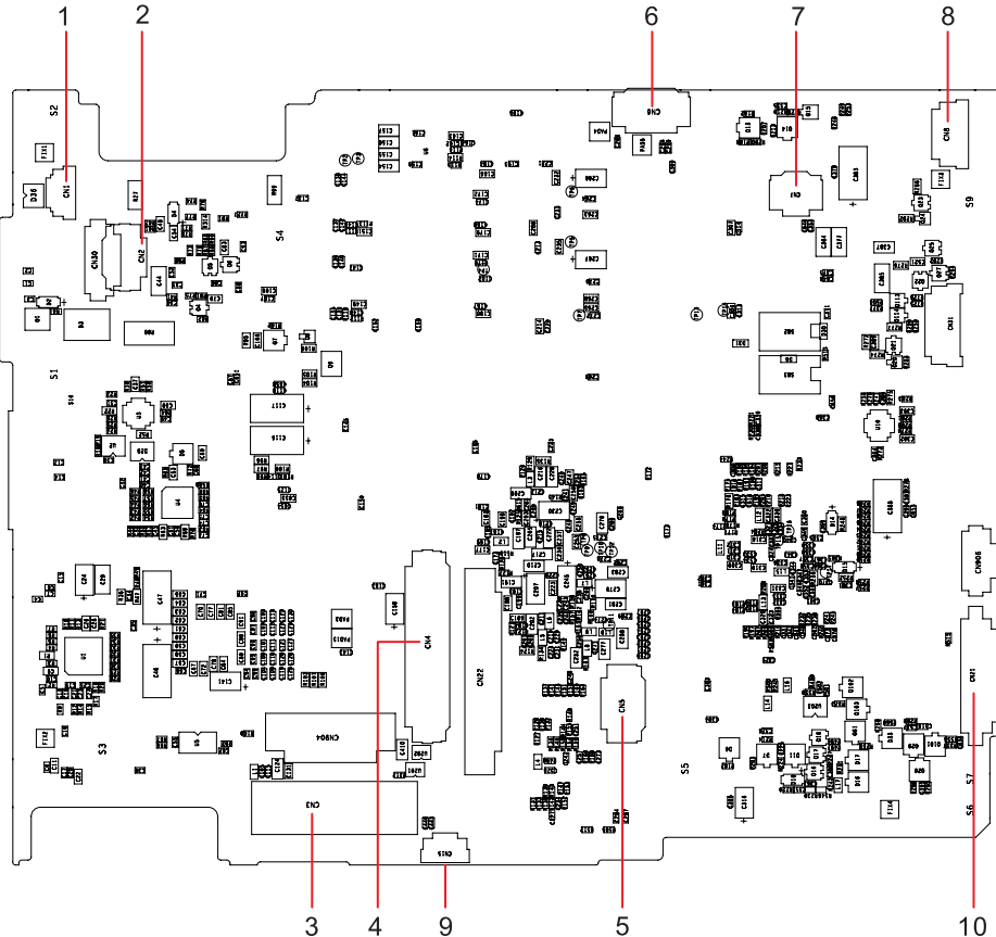
Aspire3810T/3810TG/3810TZ/3810TZG M/B layout and connector location TOP view
